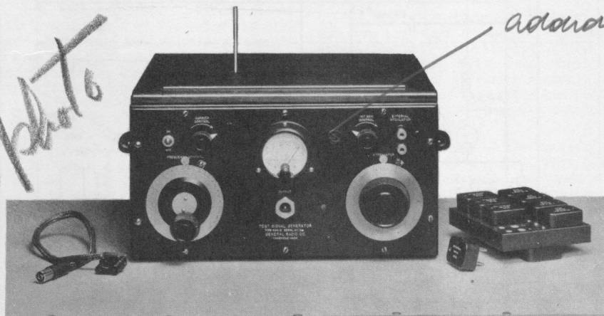
FIGURE 1. Type 604-B Test-Signal Generator showing the smallest of the three rod-type antennas in place
